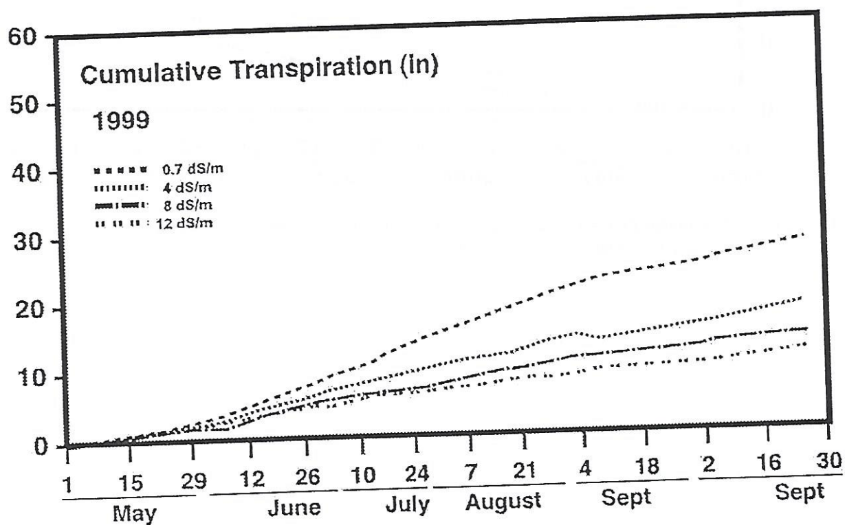
Figure 13a. Comparative seasonal transpiration for all treatments as determined by soil water content depletion between irrigations.
