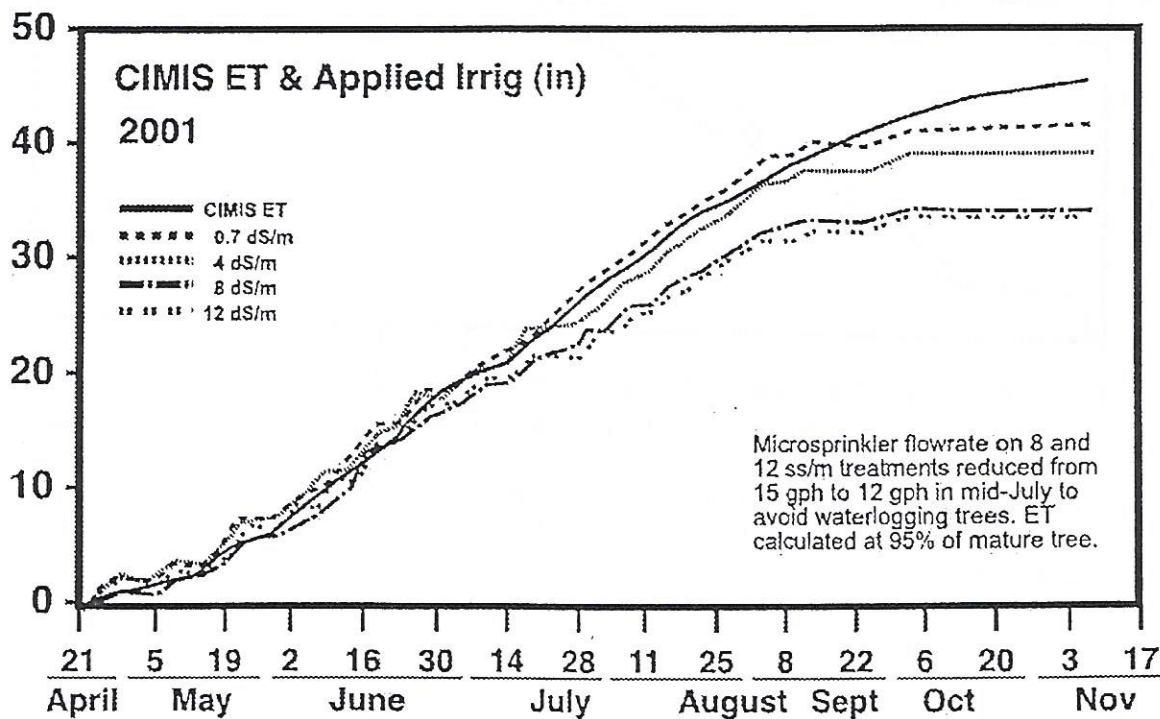
Figure 9c. Cumulative seasonal applied irrigation water to all treatments and calculated pistachio ET using 2001 CIMIS ET_0 as measured at the Shafter Field Station multiplied by crop coefficients described by Goldhamer (1987).
