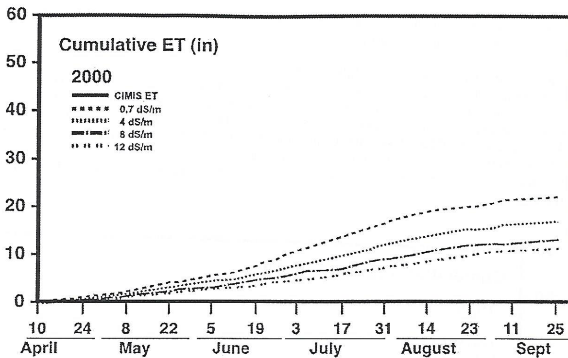
Figure 13b. Comparative seasonal evapotranspiration for all treatments as determined by soil water content depletion between irrigations.
