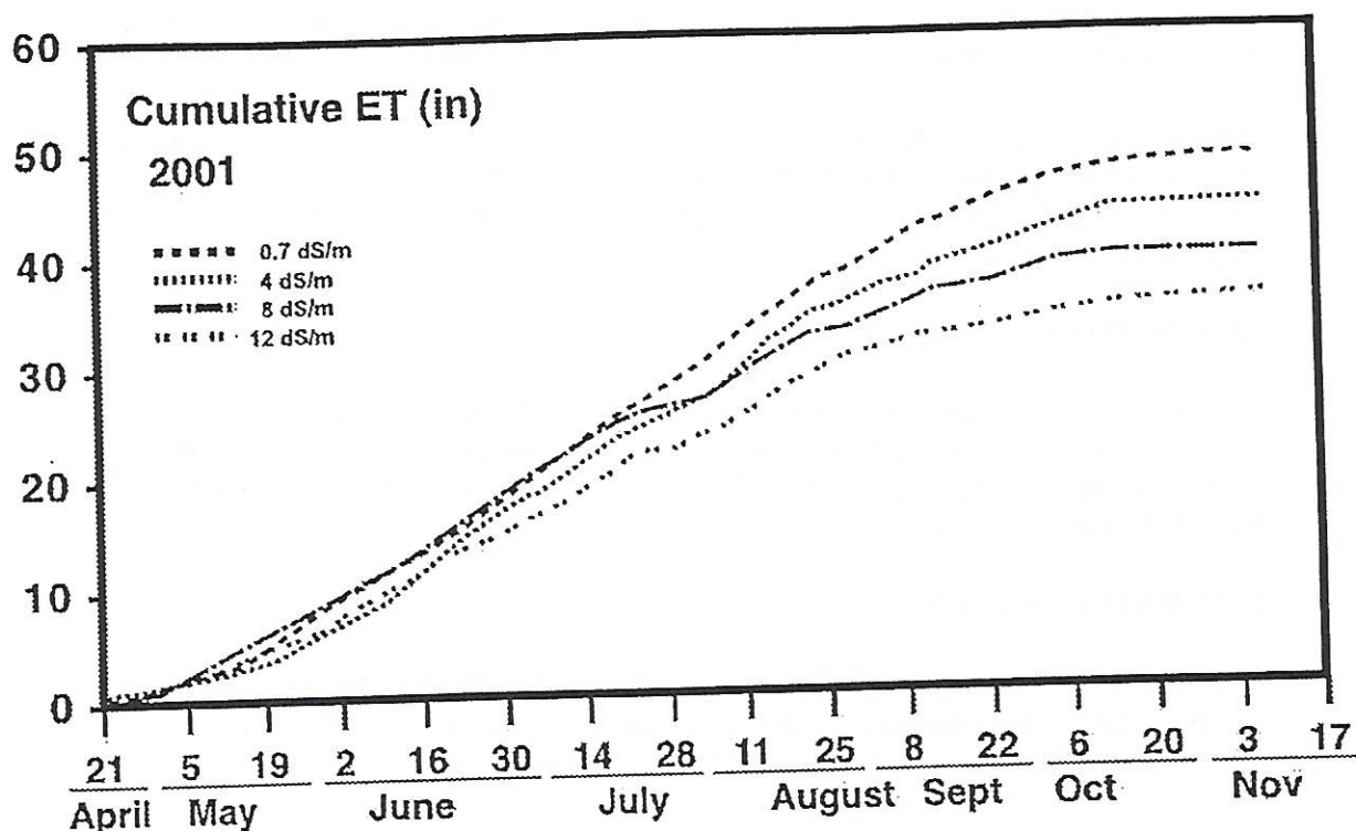
Figure 13c. Comparative seasonal evapotranspiration for all treatments as determined by soil water content depletion between irrigations and local CIMIC station evaporation.
