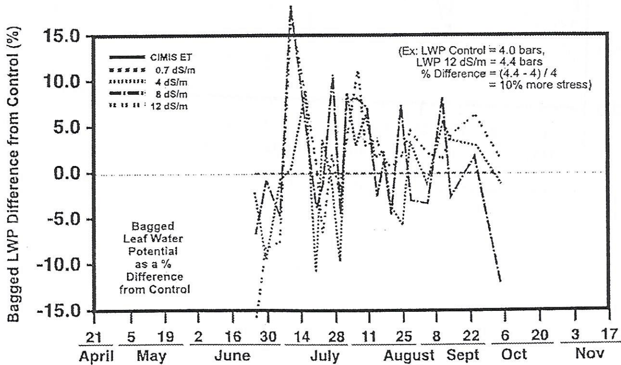
Figure 10c. Bagged midday leaf water potentials demonstrating percentage difference from the control among treatments.
