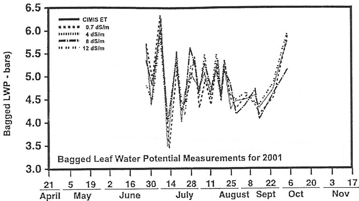
Figure 10b. Bagged midday leaf water potentials for 2001.
