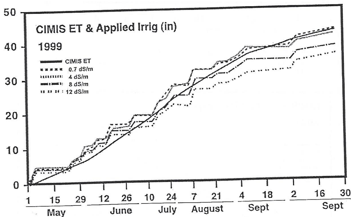
Figure 9a. Cumulative seasonal applied irrigation water to all treatments and calculated pistachio ET using 1999 CIMIS ET_0 as measured at the Shafter Field Station multiplied by crop coefficients described by Goldhamer (1987).
