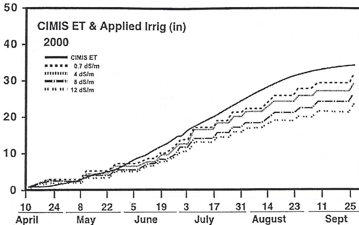
Figure 9b. Cumulative seasonal applied irrigation water to all treatments and calculated pistachio ET using 2000 CIMIS ET_0 as measured at the Shafter Field Station multiplied by crop coefficients described by Goldhamer (1987).
